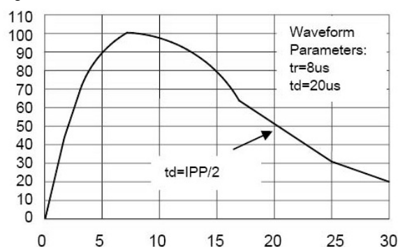
Fig1. Pulse Waveform
